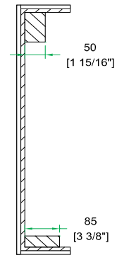
B-B VIEW
