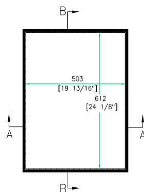
TOP VIEW OF COVER
