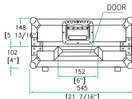
BACK VIEW
