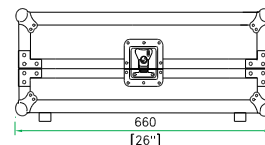
RIGHT VIEW
