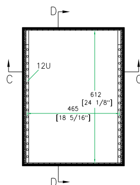
TOP VIEW OF BASE
