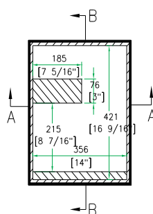
TOP VIEW OF COVER
