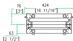
BACK VIEW
