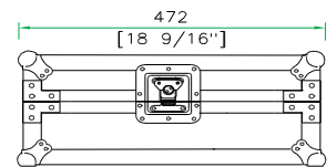
RIGHT VIEW
