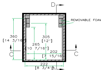
TOP VIEW OF BASE
